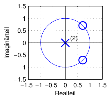
System III ROC: |z| > 0
