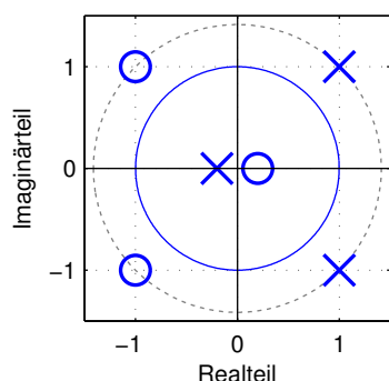
System I ROC: \frac{1}{5} < |z| < \sqrt{2}
