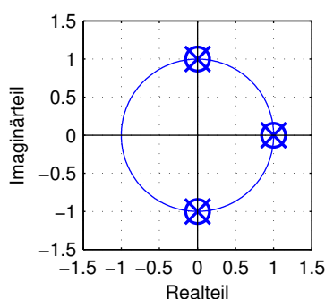
System II ROC: 1 < |z| < \infty
