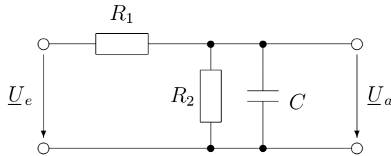
Abbildung 7: Passives Filter
