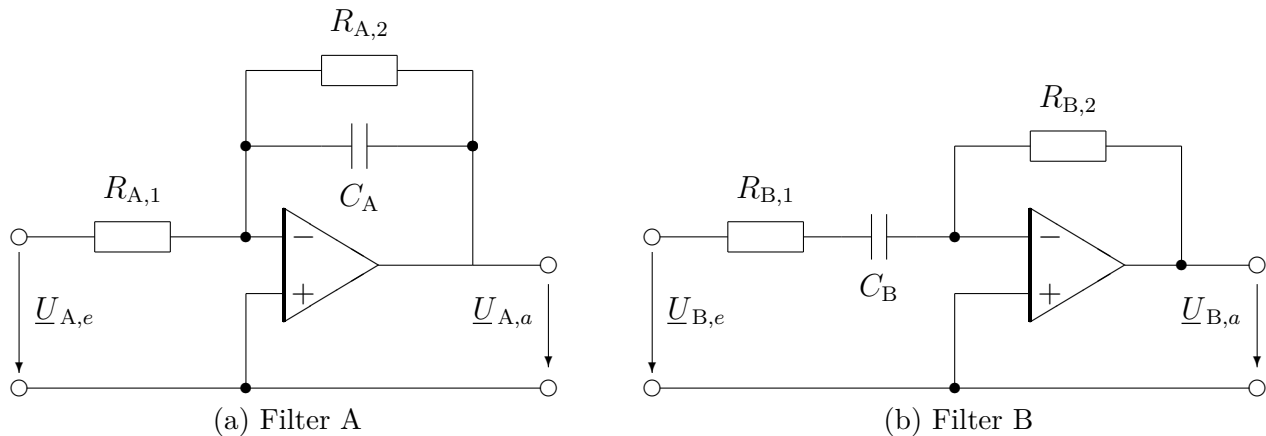
Abbildung 6: Aktive Filter
