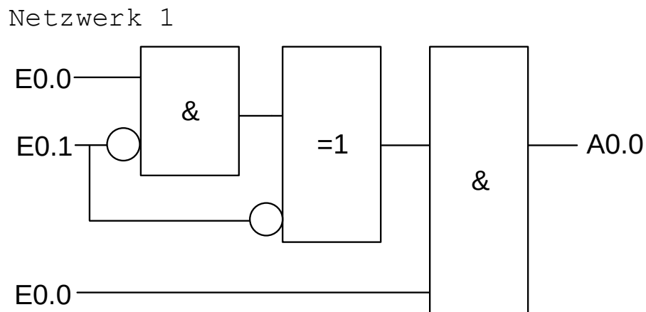
Abbildung 7: SPS-Programm in FUP
